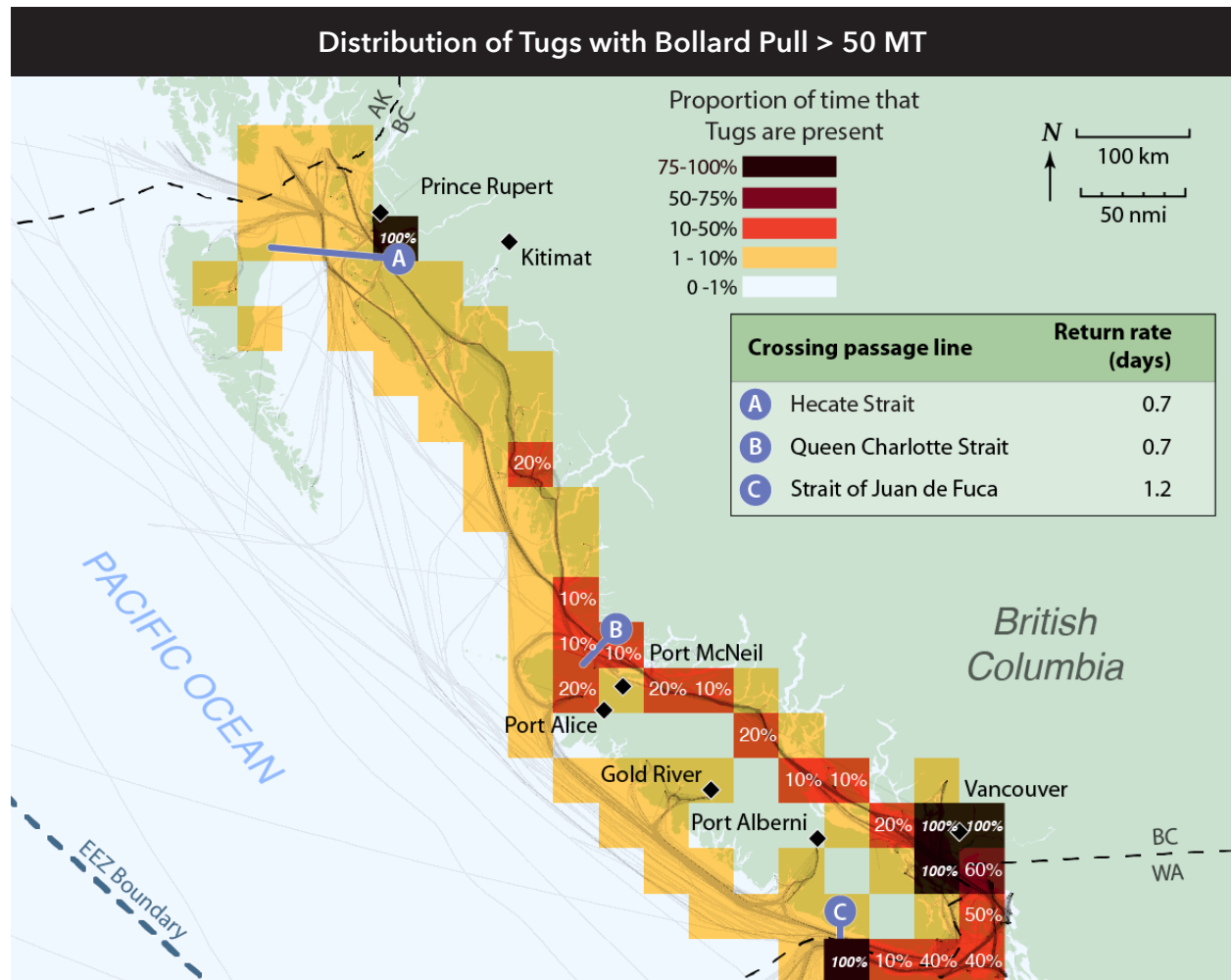
Figure 3. Average proportion of time tugs are present and return rate for tugs with a bollard pull greater than 50 MT identified by AIS in the study area in 2016.
